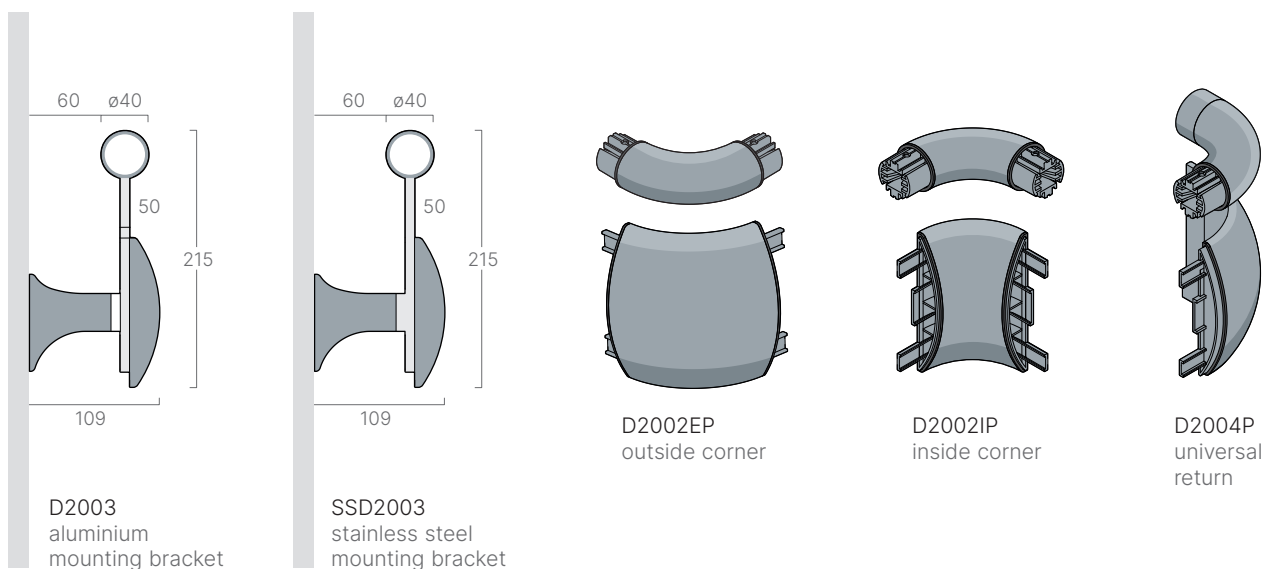
D200P PVC-u wall guard with PVC-u handrail and PVC-u accessories
